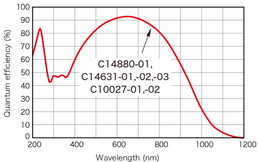
BT- CCD linear image sensor
